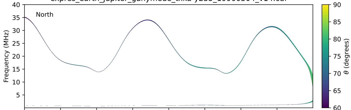
expres_earth_jupiter_ganymede_txka-y235_19900304_v14.cdf
