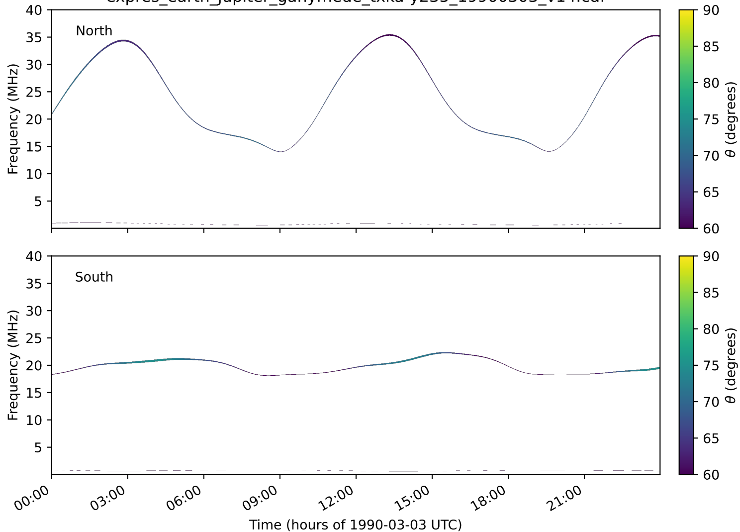
expres_earth_jupiter_ganymede_txka-y235_19900303_v14.cdf
