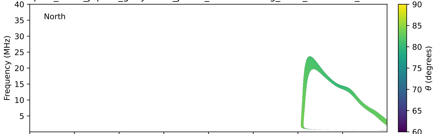
expres_earth_jupiter_ganymede_jrm33_lossc-wid1deg_3kev_19900323_v11.cdf
