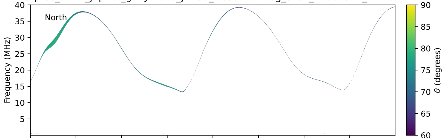
expres_earth_jupiter_ganymede_jrm09_lossc-wid1deg_3kev_19900317_v11.cdf
