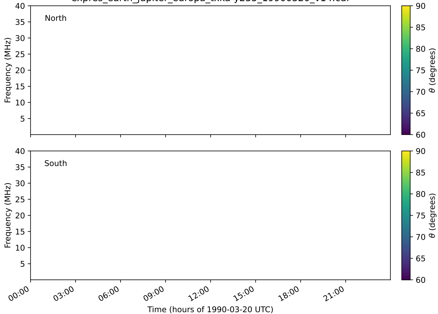
expres_earth_jupiter_europa_txka-y235_19900320_v14.cdf
