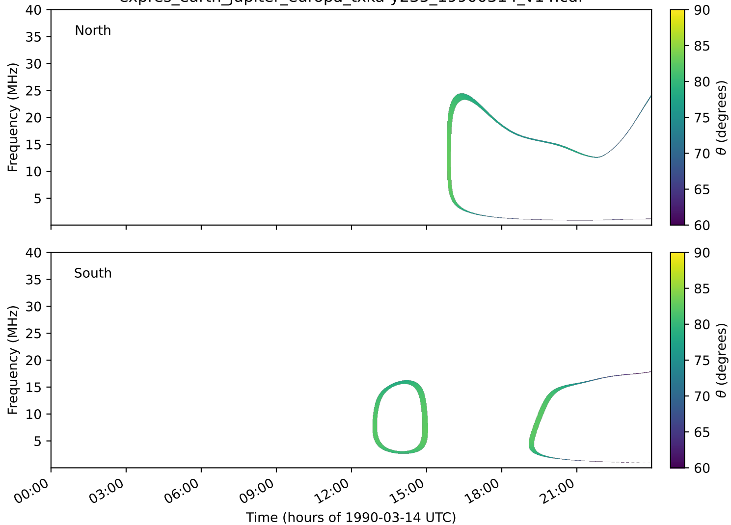
expres_earth_jupiter_europa_txka-y235_19900314_v14.cdf
