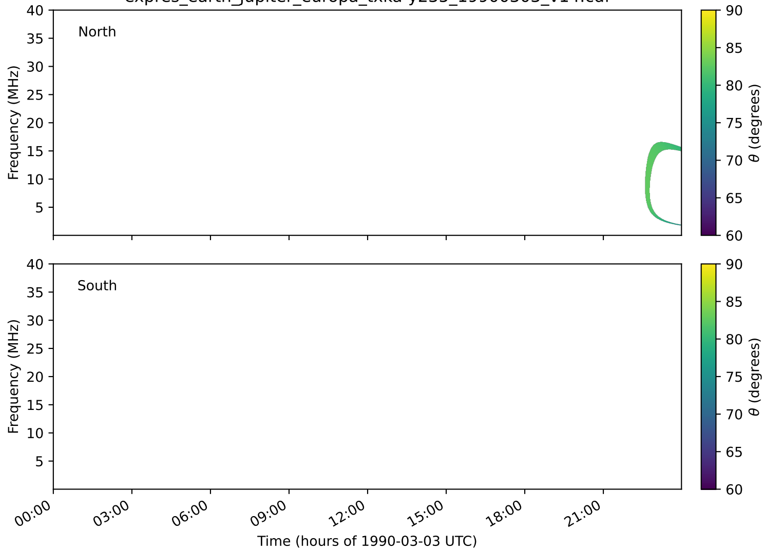
expres_earth_jupiter_europa_txka-y235_19900303_v14.cdf
