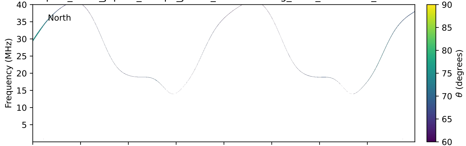
expres_earth_jupiter_europa_jrm33_lossc-wid1deg_3kev_19900315_v11.cdf
