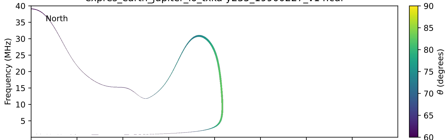
expres_earth_jupiter_io_txka-y235_19900227_v14.cdf
