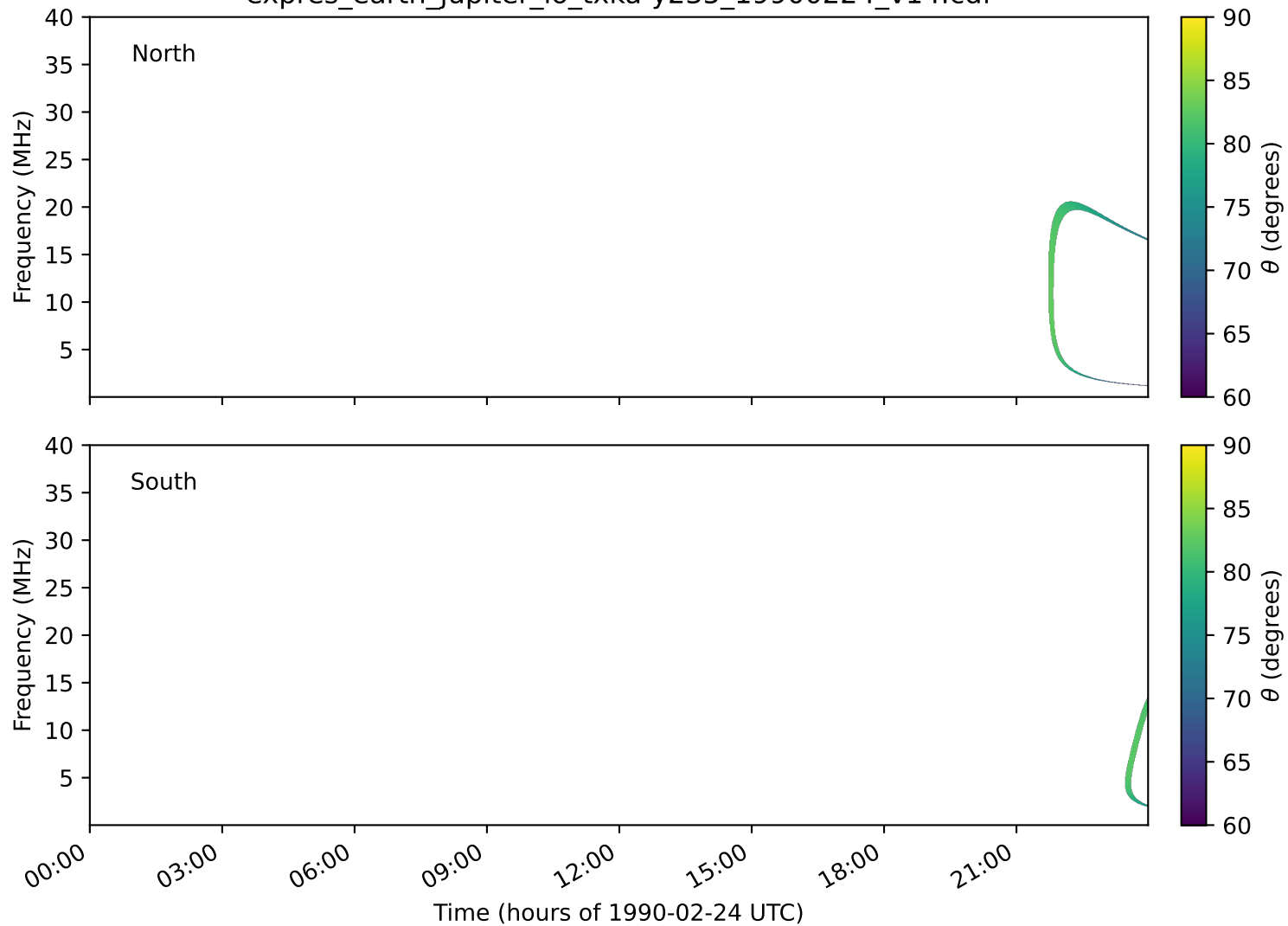
expres_earth_jupiter_io_txka-y235_19900224_v14.cdf
