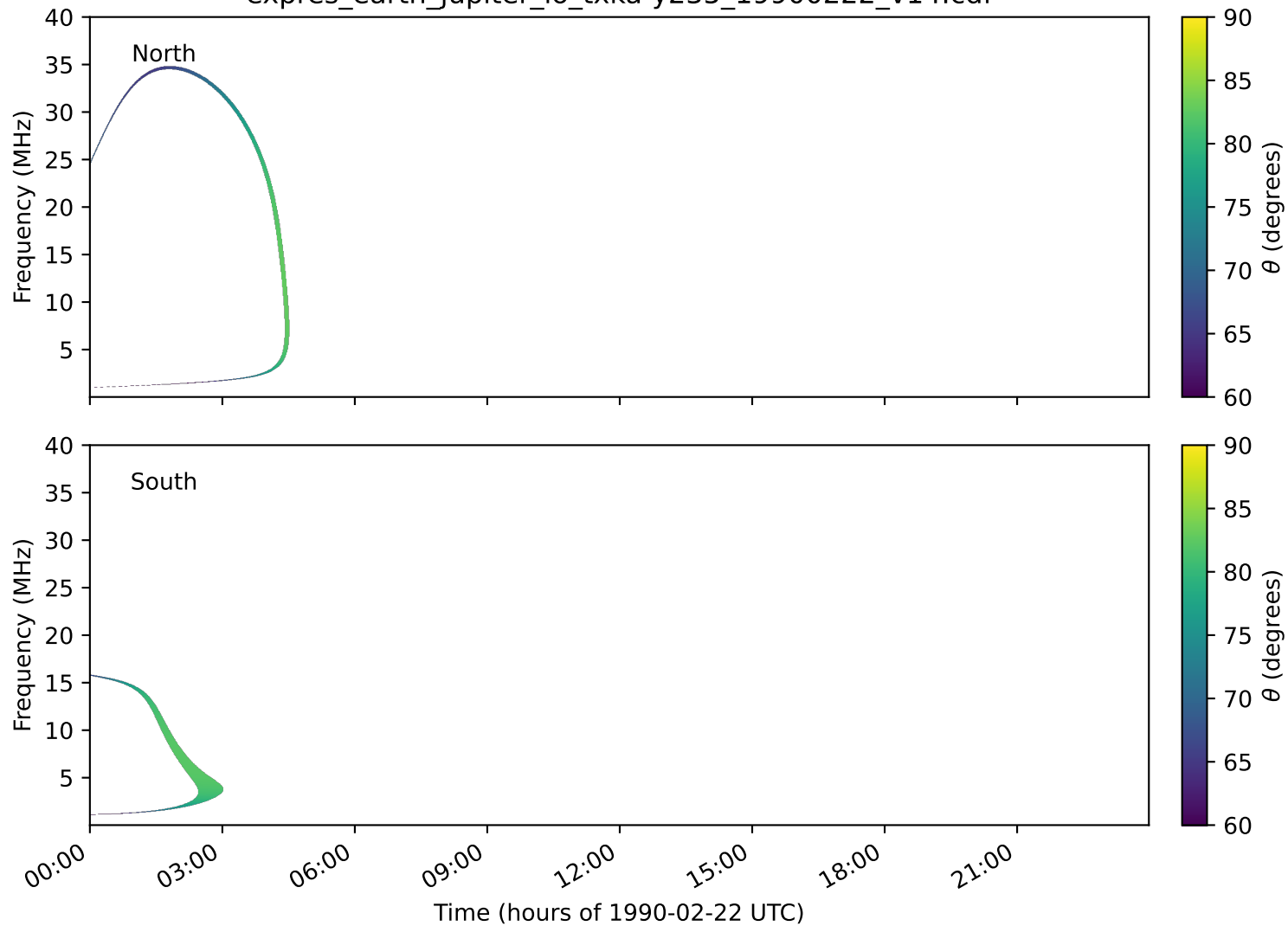
expres_earth_jupiter_io_txka-y235_19900222_v14.cdf
