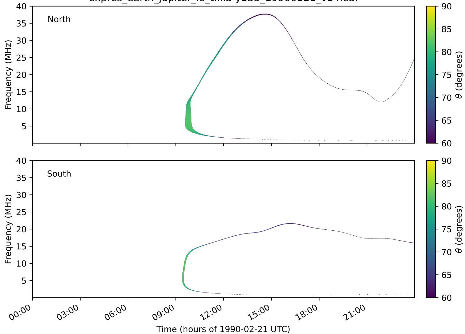
expres_earth_jupiter_io_txka-y235_19900221_v14.cdf
