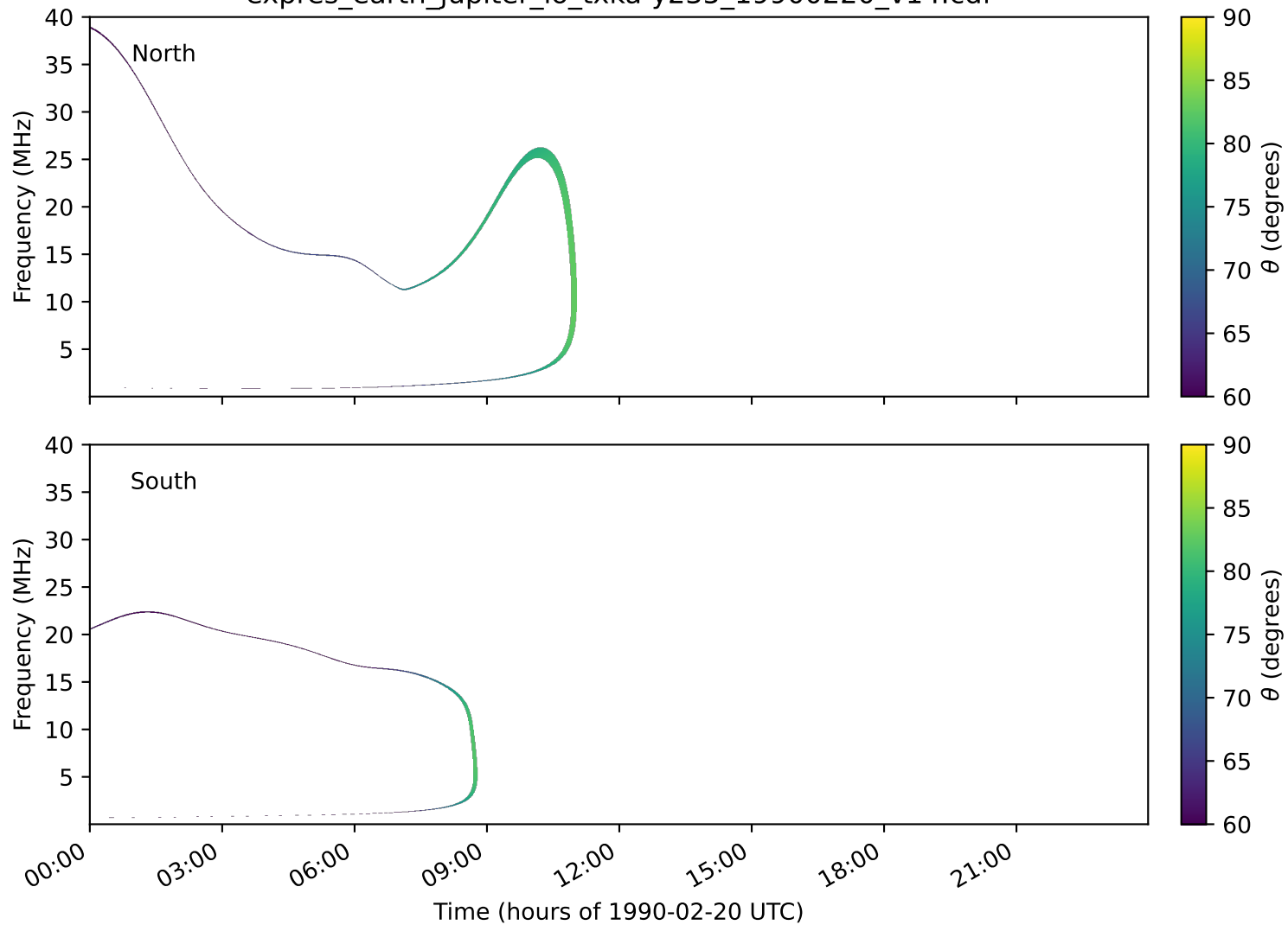
expres_earth_jupiter_io_txka-y235_19900220_v14.cdf
