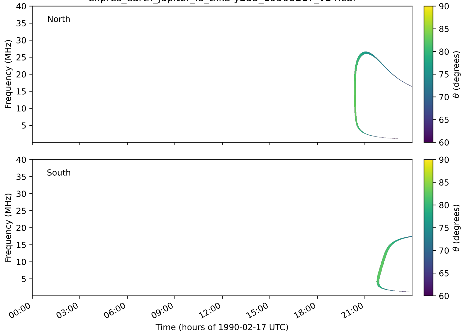
expres_earth_jupiter_io_txka-y235_19900217_v14.cdf
