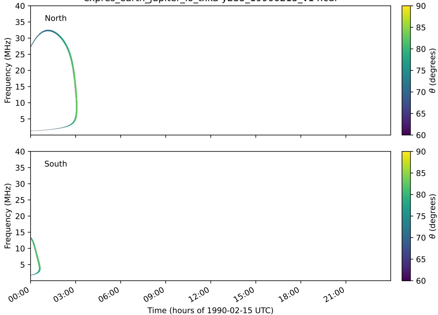
expres_earth_jupiter_io_txka-y235_19900215_v14.cdf
