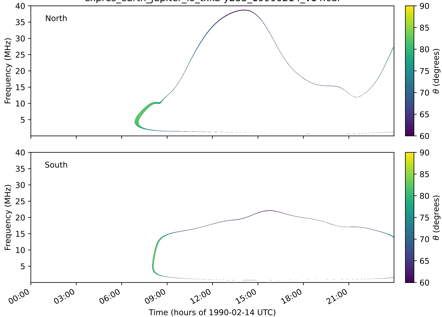
expres_earth_jupiter_io_txka-y235_19900214_v14.cdf
