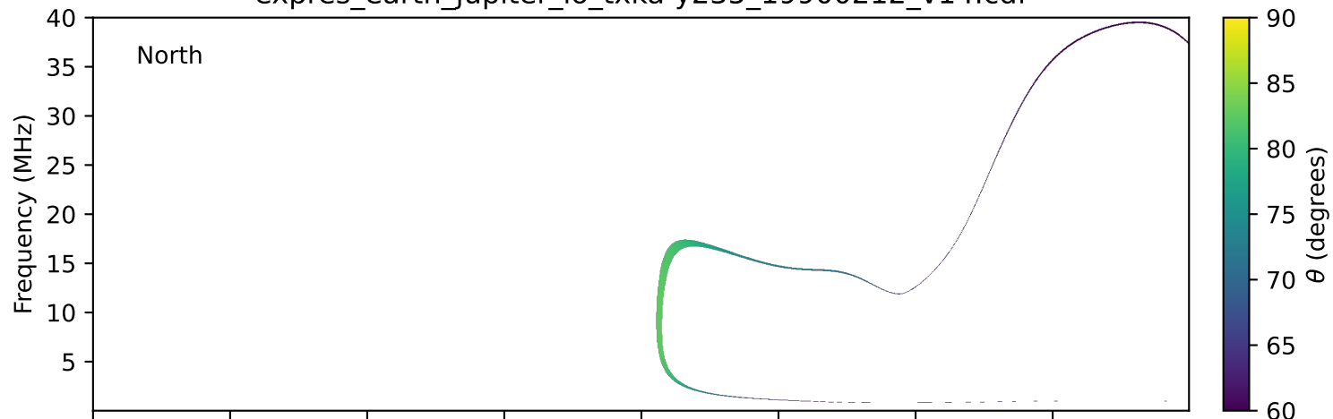
expres_earth_jupiter_io_txka-y235_19900212_v14.cdf
