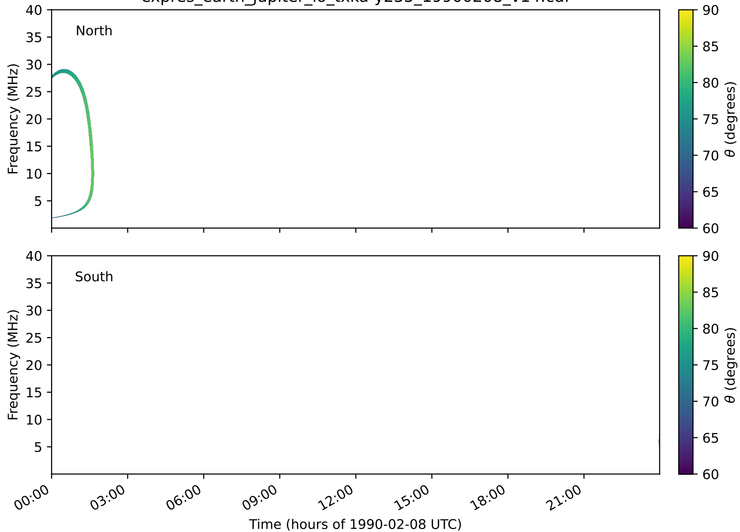
expres_earth_jupiter_io_txka-y235_19900208_v14.cdf
