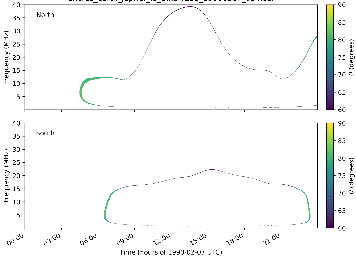
expres_earth_jupiter_io_txka-y235_19900207_v14.cdf
