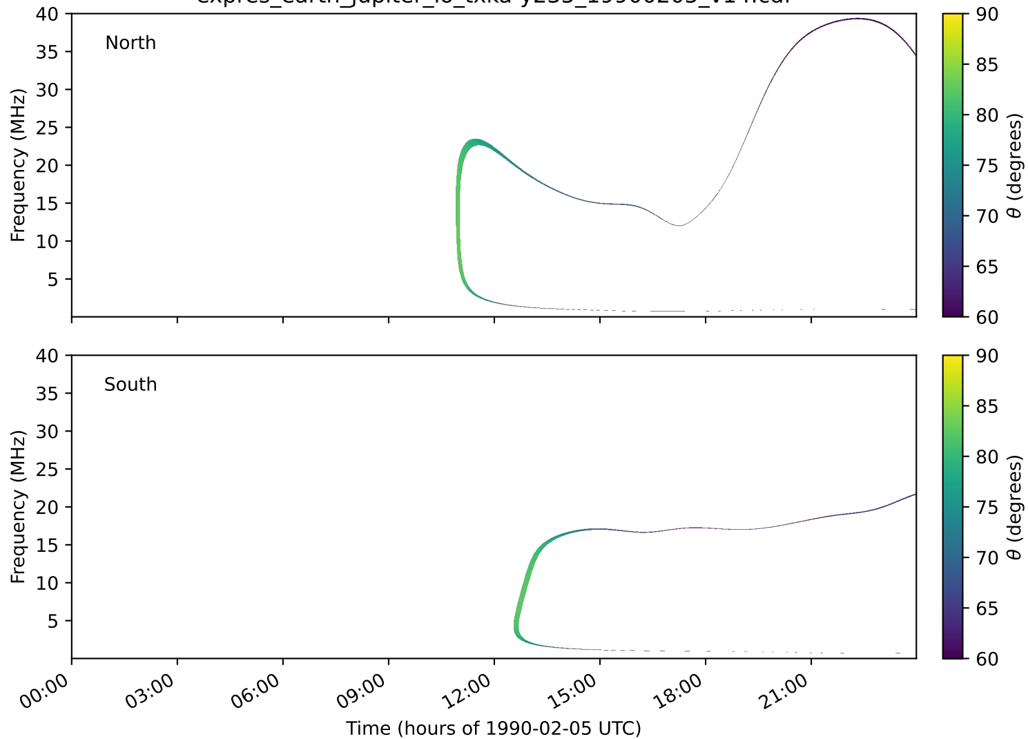
expres_earth_jupiter_io_txka-y235_19900205_v14.cdf
