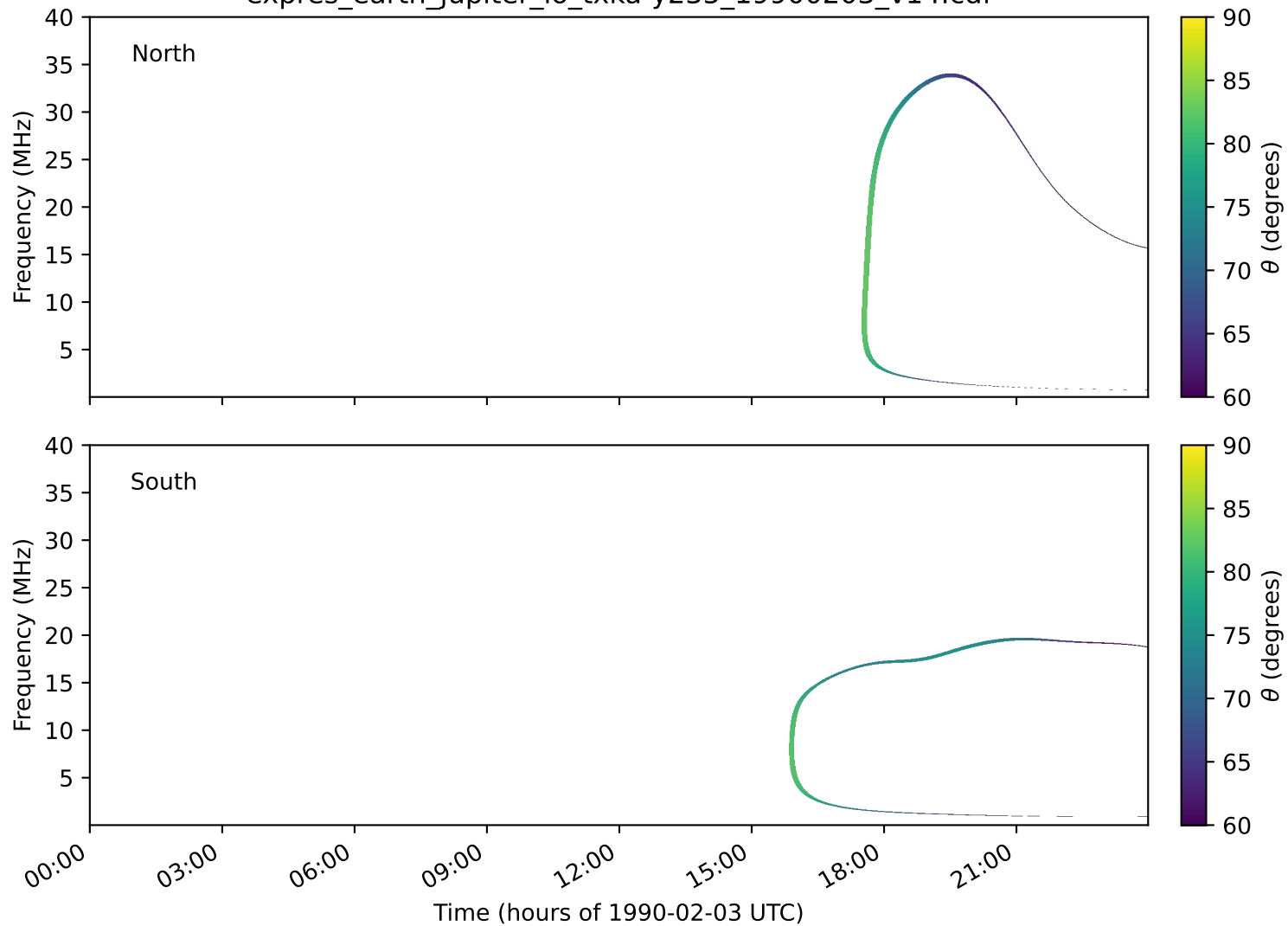
expres_earth_jupiter_io_txka-y235_19900203_v14.cdf
