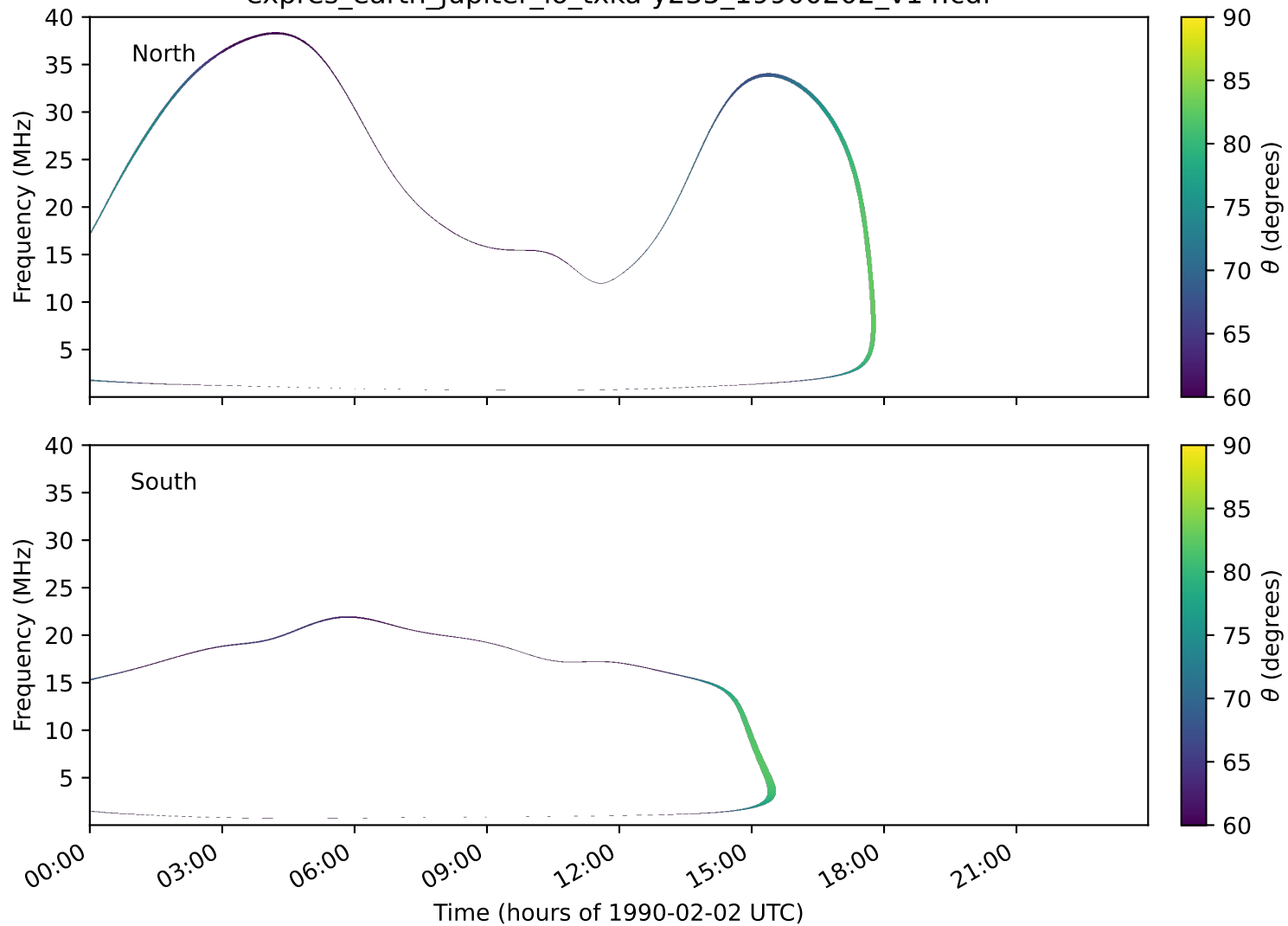
expres_earth_jupiter_io_txka-y235_19900202_v14.cdf
