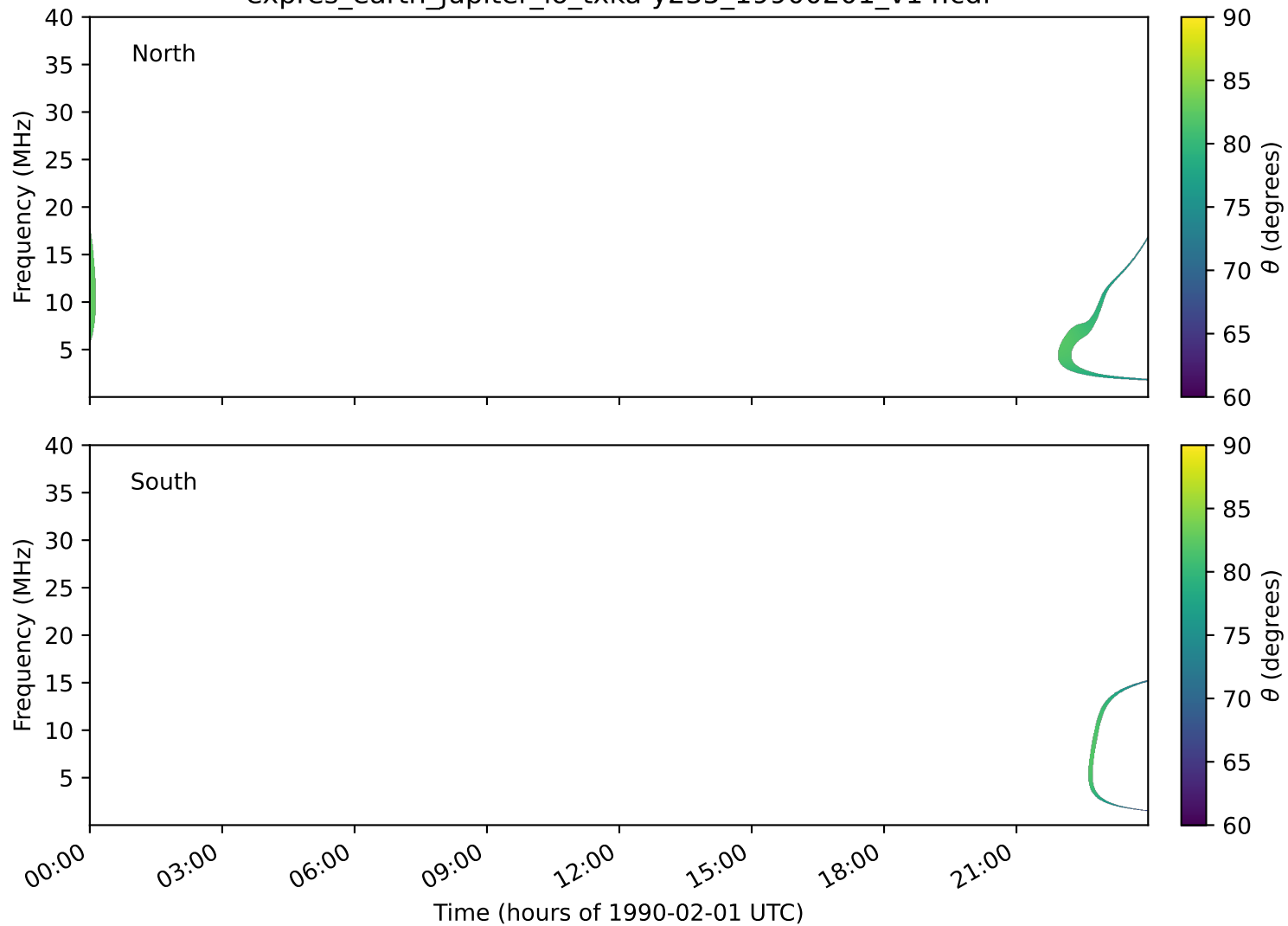
expres_earth_jupiter_io_txka-y235_19900201_v14.cdf
