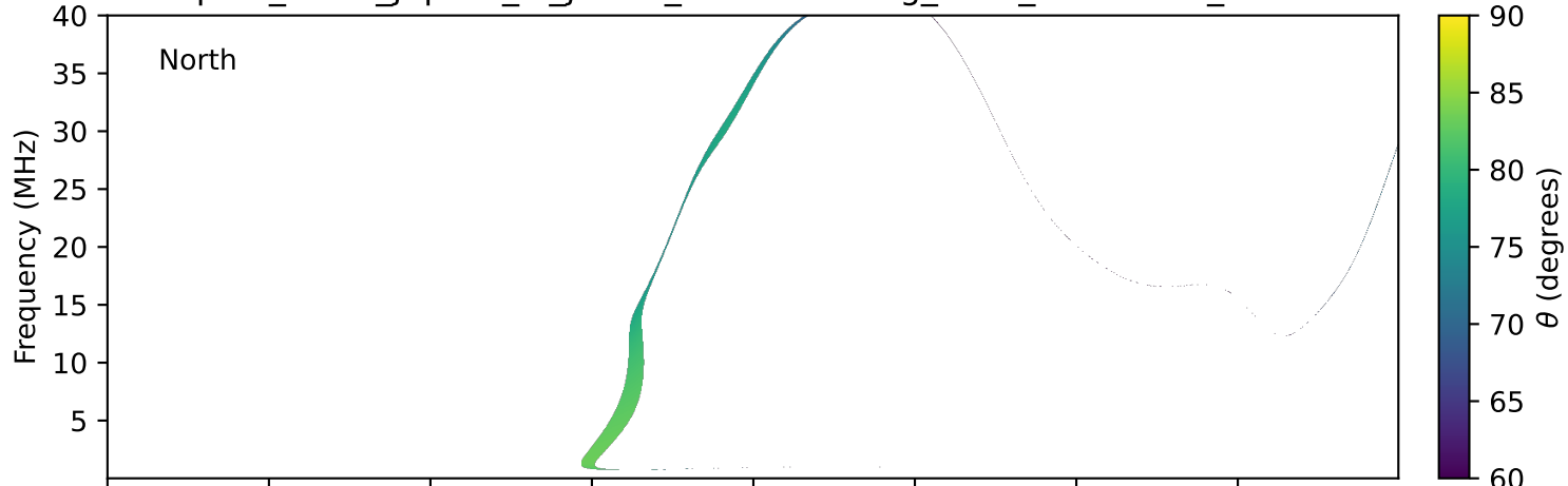
expres_earth_jupiter_io_jrm33_lossc-wid1deg_3kev_19900221_v11.cdf
