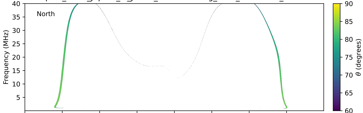
expres_earth_jupiter_io_jrm33_lossc-wid1deg_3kev_19900216_v11.cdf
