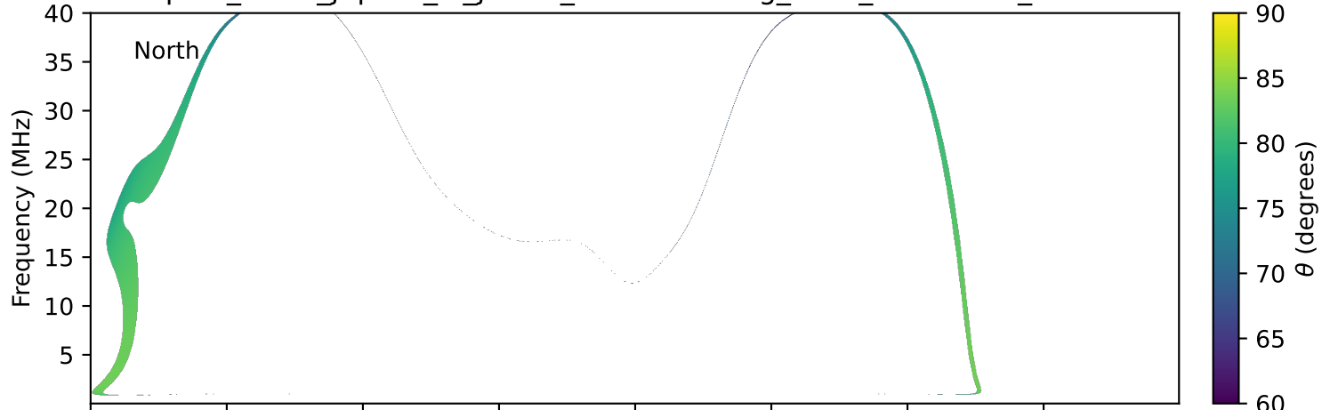
expres_earth_jupiter_io_jrm33_lossc-wid1deg_3kev_19900209_v11.cdf
