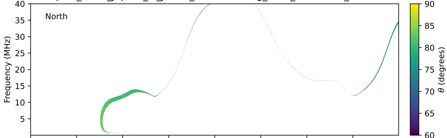
expres_earth_jupiter_io_jrm33_lossc-wid1deg_3kev_19900207_v11.cdf
