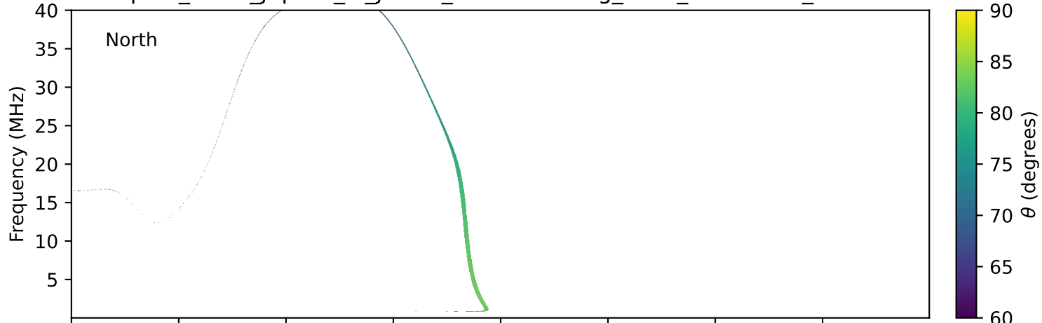
expres_earth_jupiter_io_jrm33_lossc-wid1deg_3kev_19900204_v11.cdf
