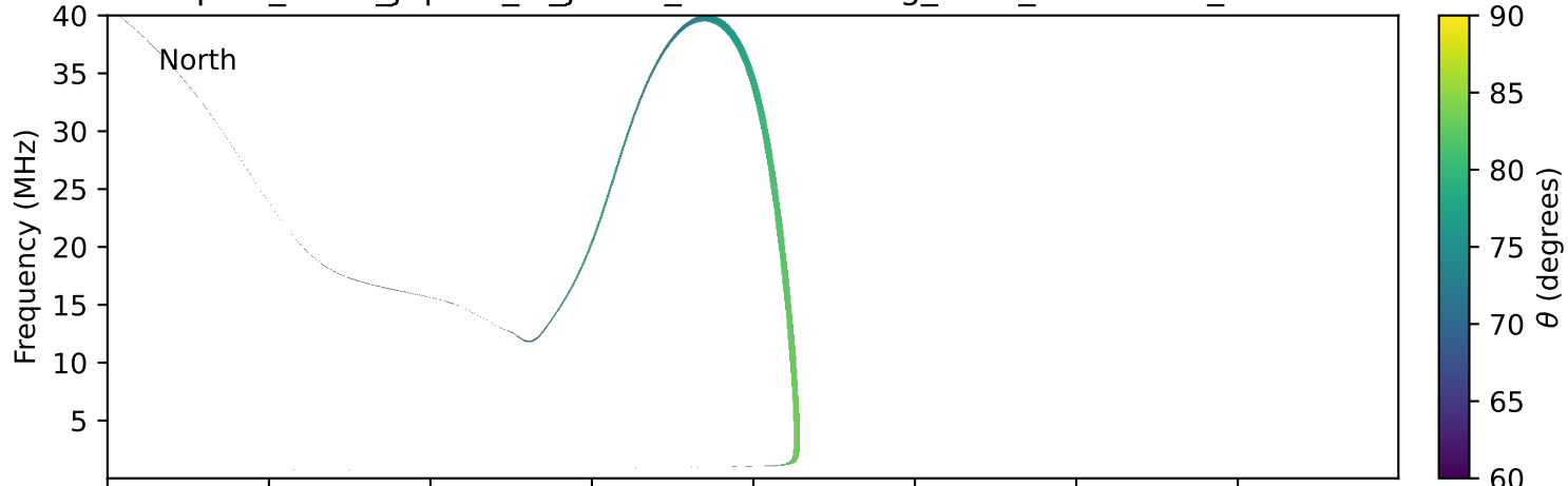
expres_earth_jupiter_io_jrm09_lossc-wid1deg_3kev_19900227_v11.cdf
