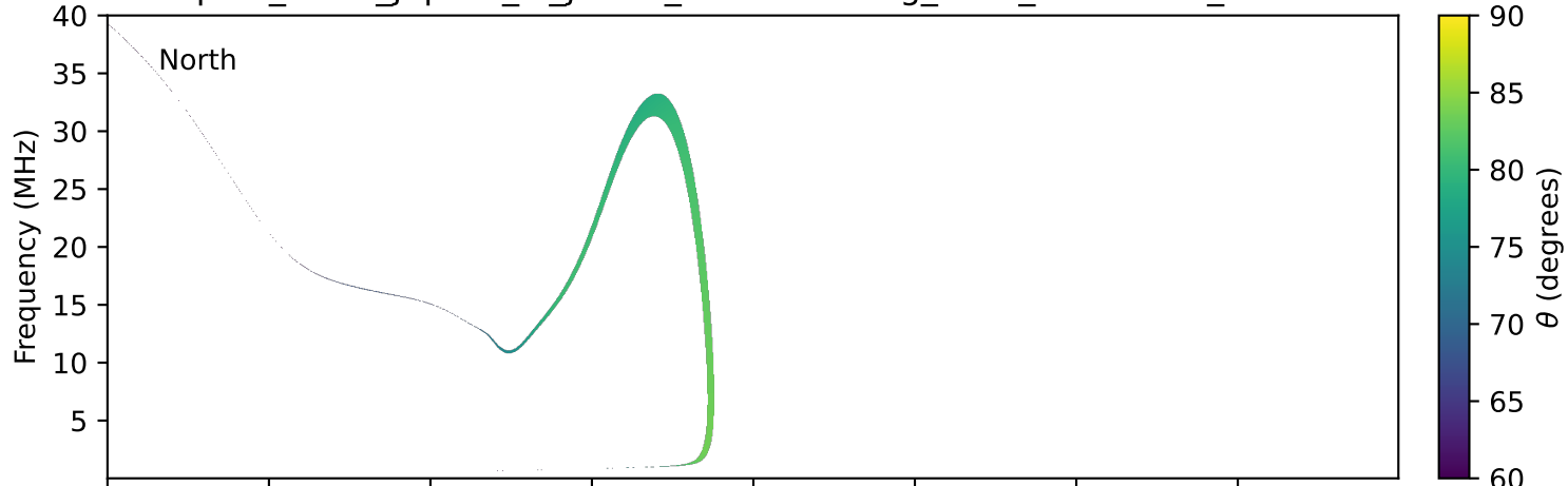
expres_earth_jupiter_io_jrm09_lossc-wid1deg_3kev_19900220_v11.cdf
