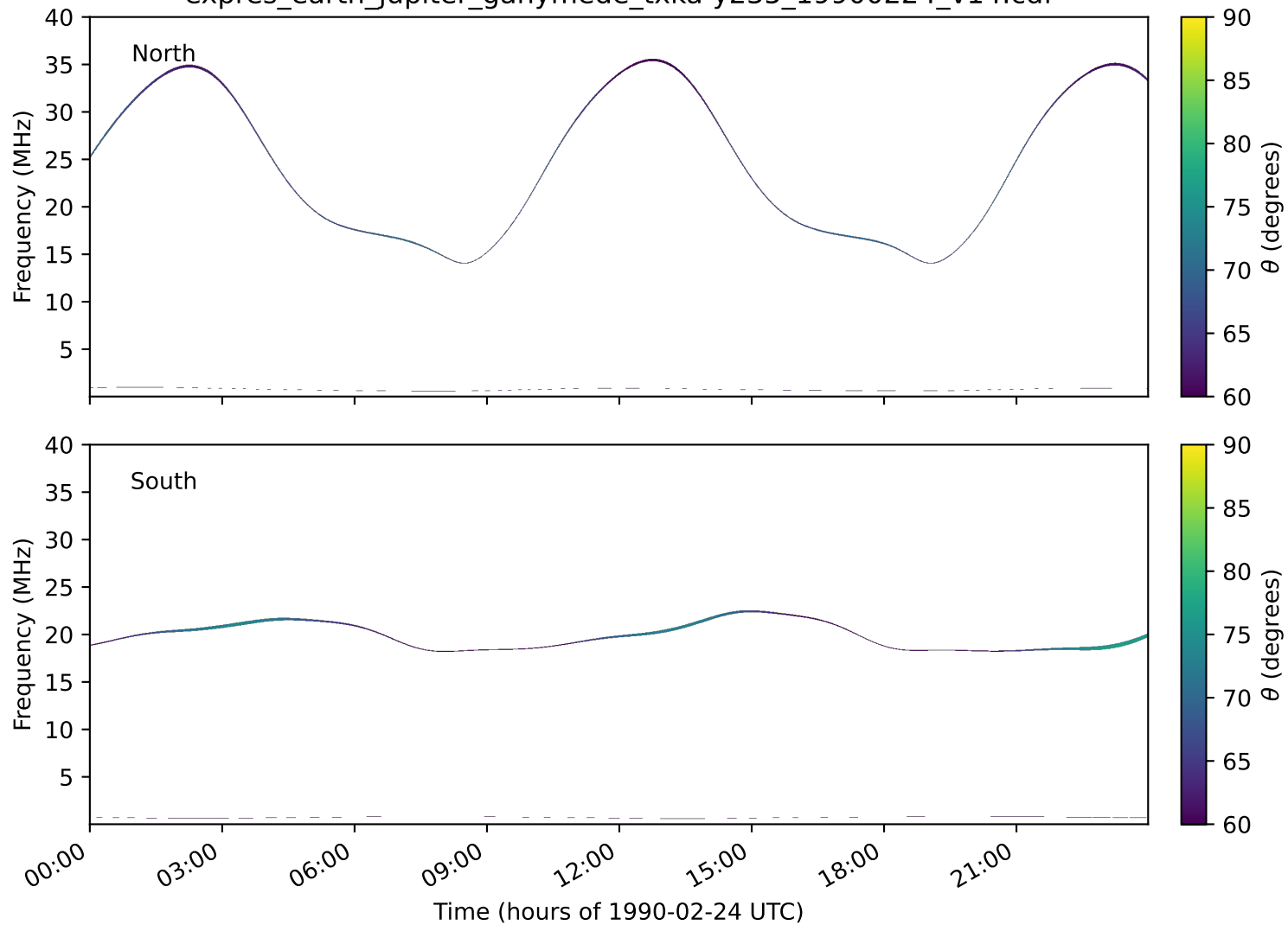
expres_earth_jupiter_ganymede_txka-y235_19900224_v14.cdf
