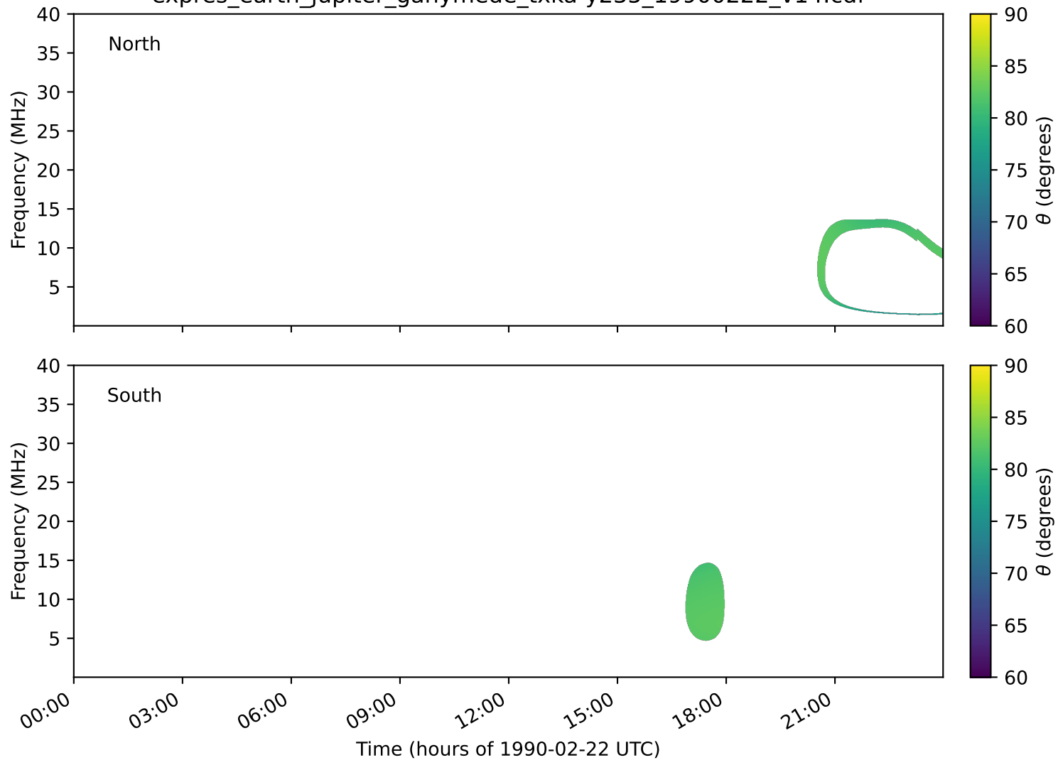
expres_earth_jupiter_ganymede_txka-y235_19900222_v14.cdf
