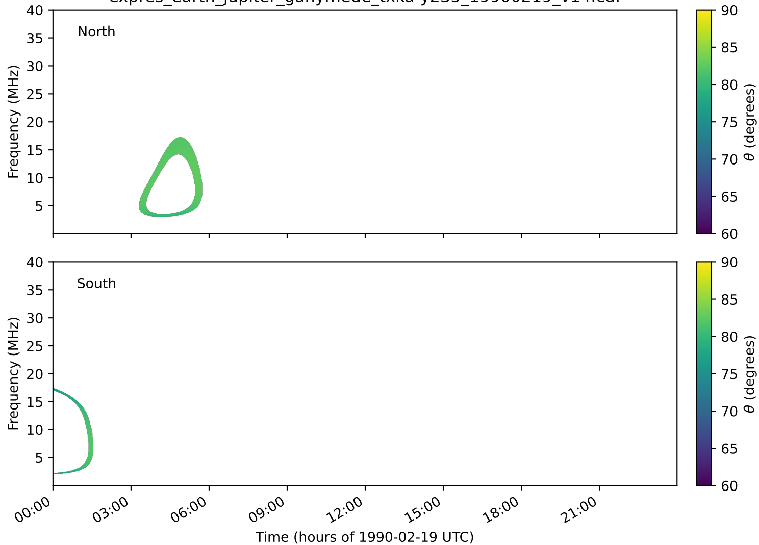
expres_earth_jupiter_ganymede_txka-y235_19900219_v14.cdf
