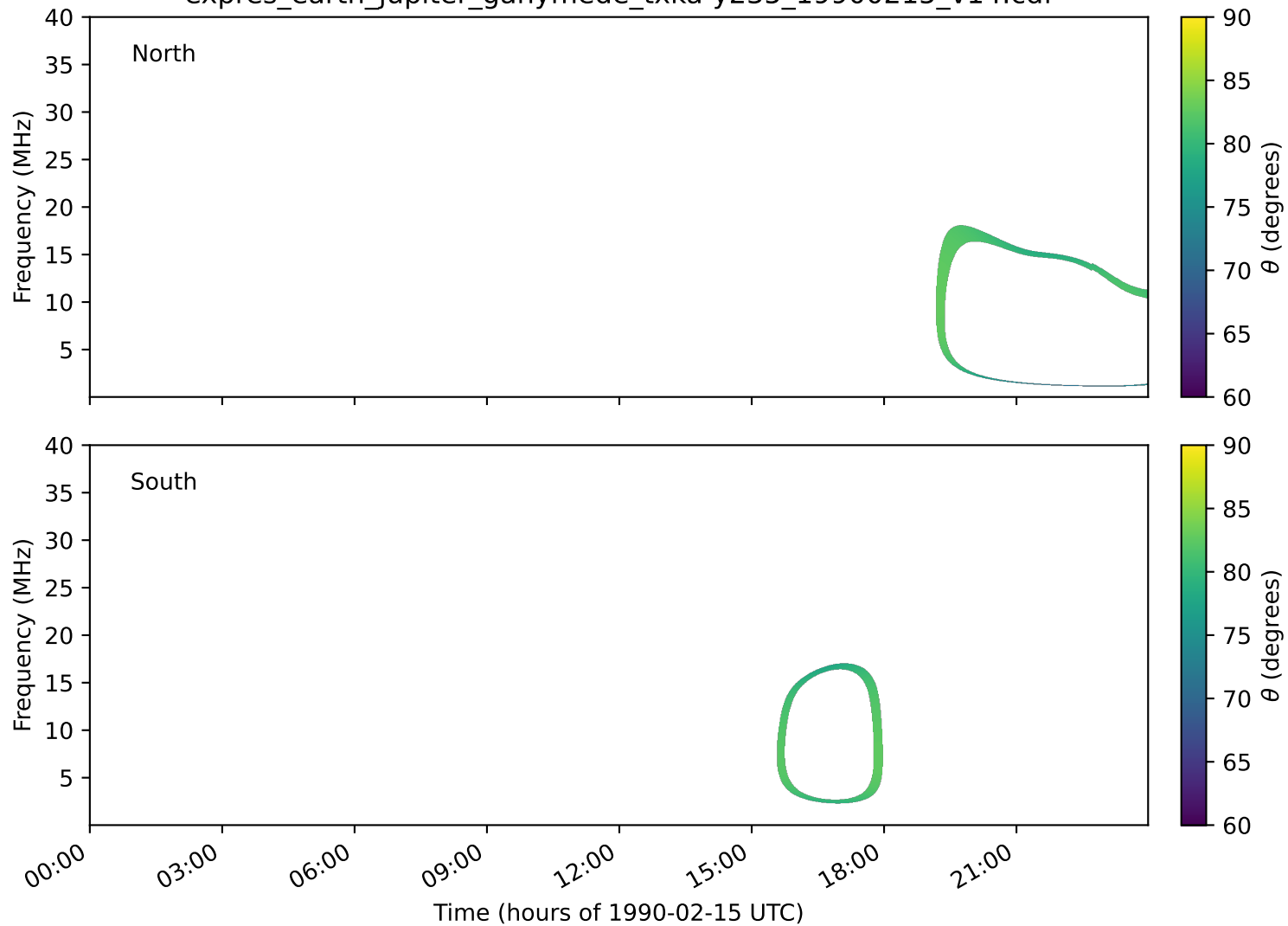
expres_earth_jupiter_ganymede_txka-y235_19900215_v14.cdf
