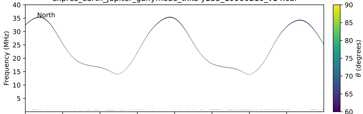
expres_earth_jupiter_ganymede_txka-y235_19900210_v14.cdf
