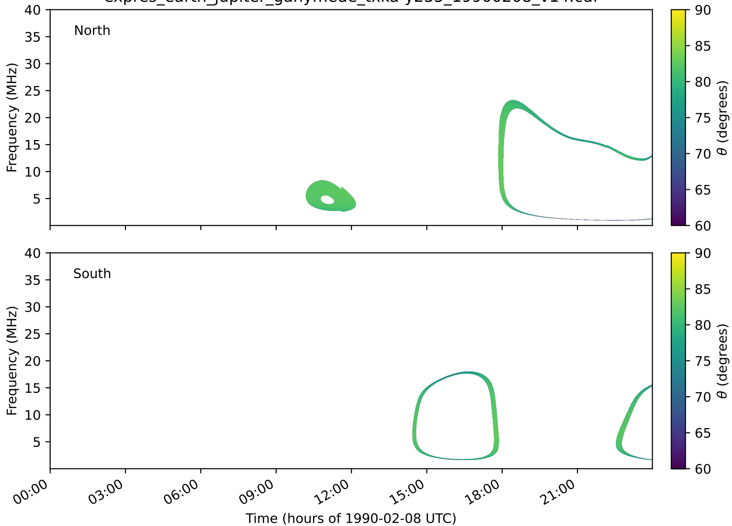
expres_earth_jupiter_ganymede_txka-y235_19900208_v14.cdf
