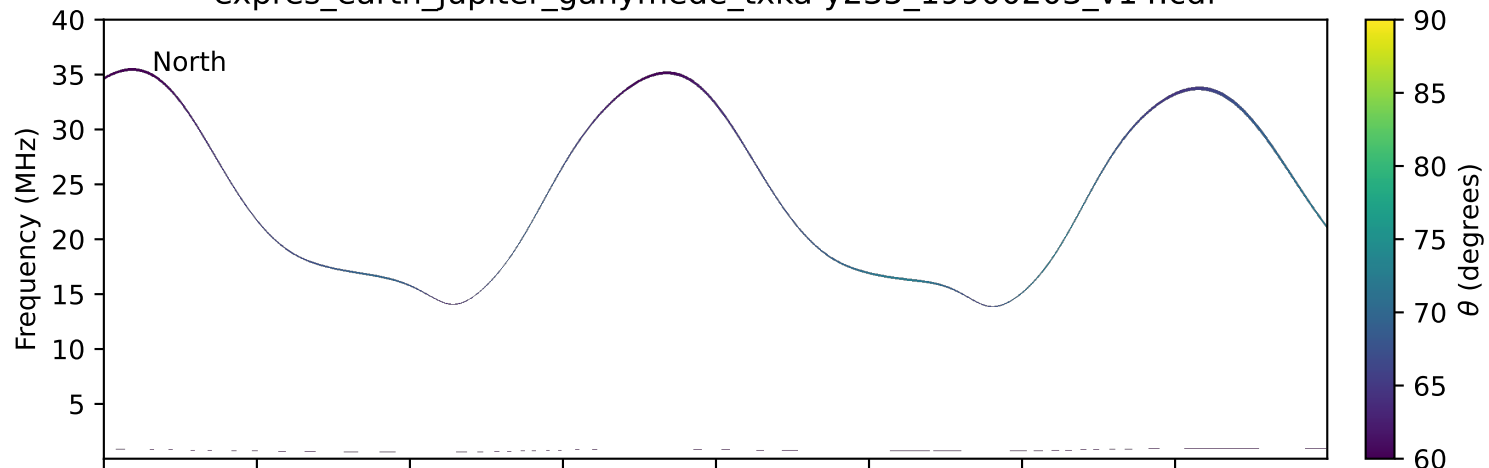
expres_earth_jupiter_ganymede_txka-y235_19900203_v14.cdf
