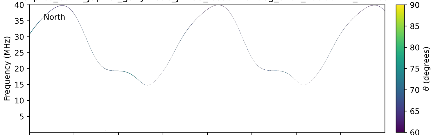
expres_earth_jupiter_ganymede_jrm33_lossc-wid1deg_3kev_19900224_v11.cdf
