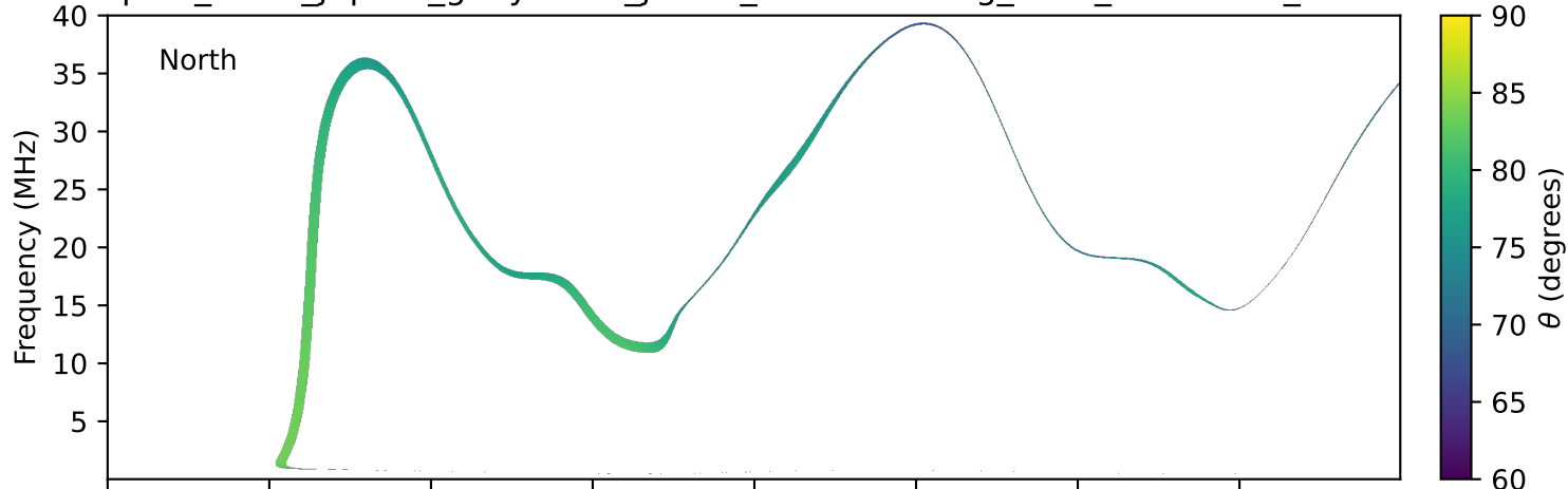
expres_earth_jupiter_ganymede_jrm33_lossc-wid1deg_3kev_19900216_v11.cdf
