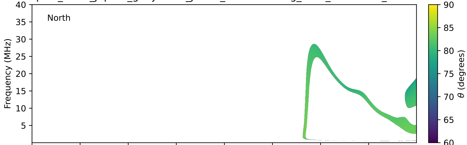
expres_earth_jupiter_ganymede_jrm33_lossc-wid1deg_3kev_19900201_v11.cdf
