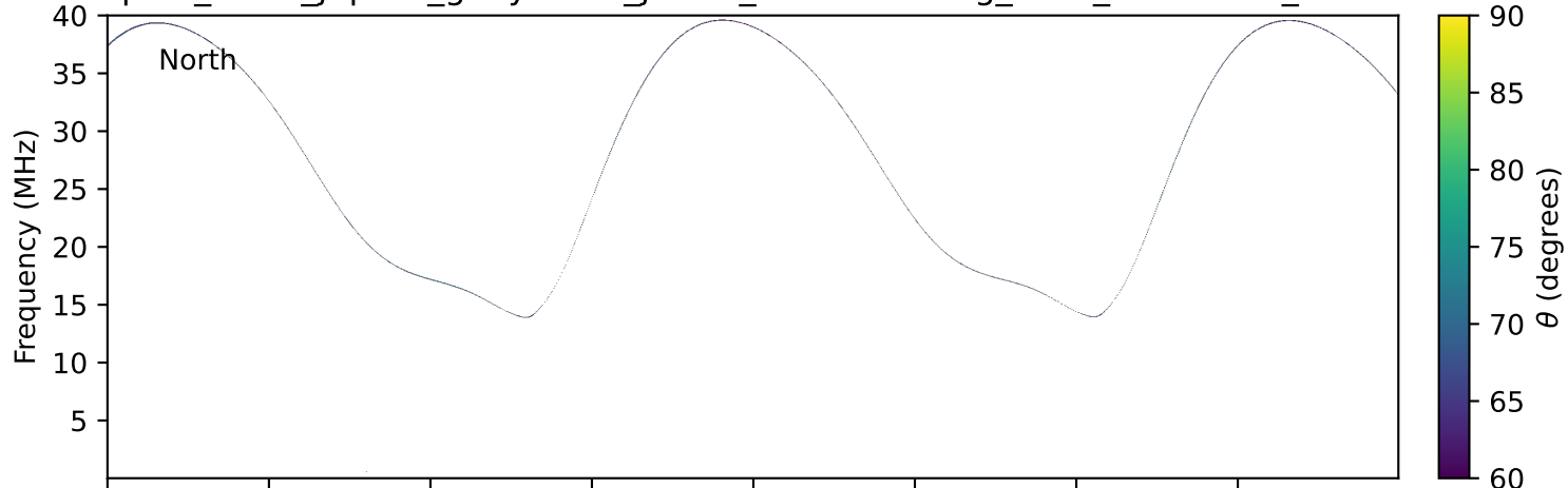
expres_earth_jupiter_ganymede_jrm09_lossc-wid1deg_3kev_19900217_v11.cdf
