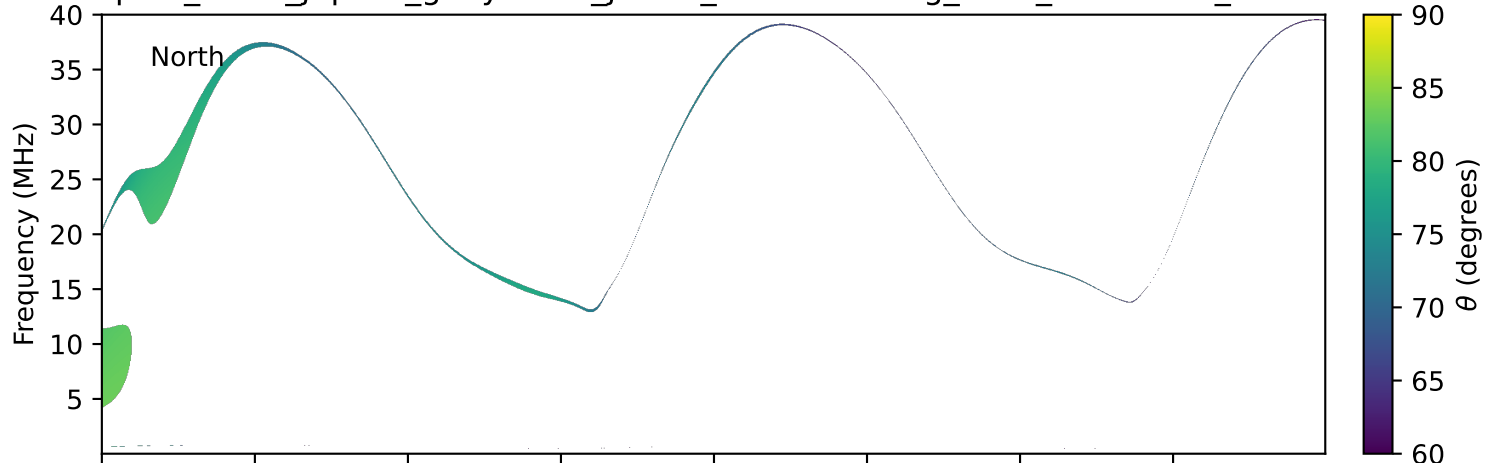
expres_earth_jupiter_ganymede_jrm09_lossc-wid1deg_3kev_19900202_v11.cdf
