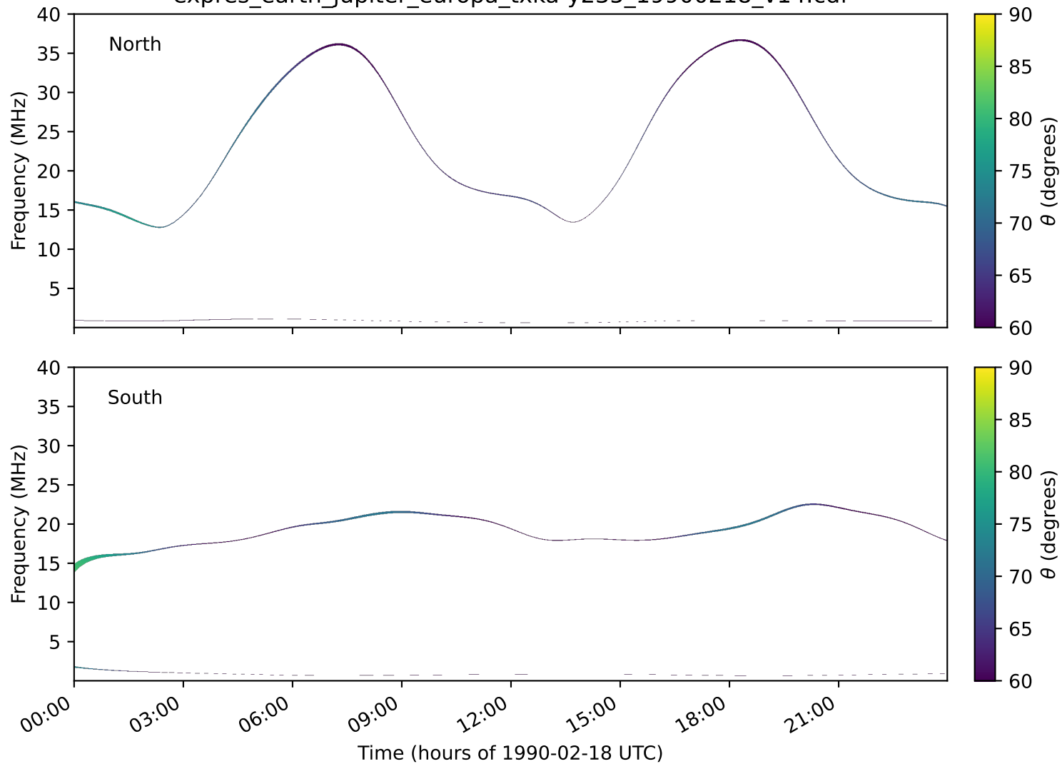
expres_earth_jupiter_europa_txka-y235_19900218_v14.cdf
