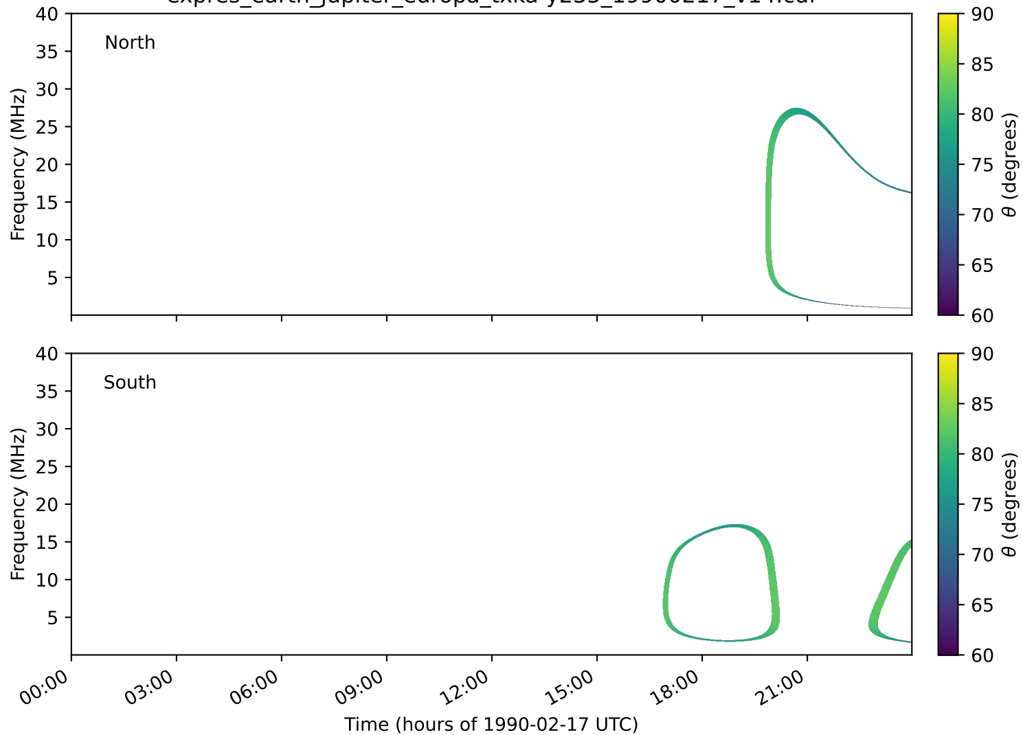
expres_earth_jupiter_europa_txka-y235_19900217_v14.cdf
