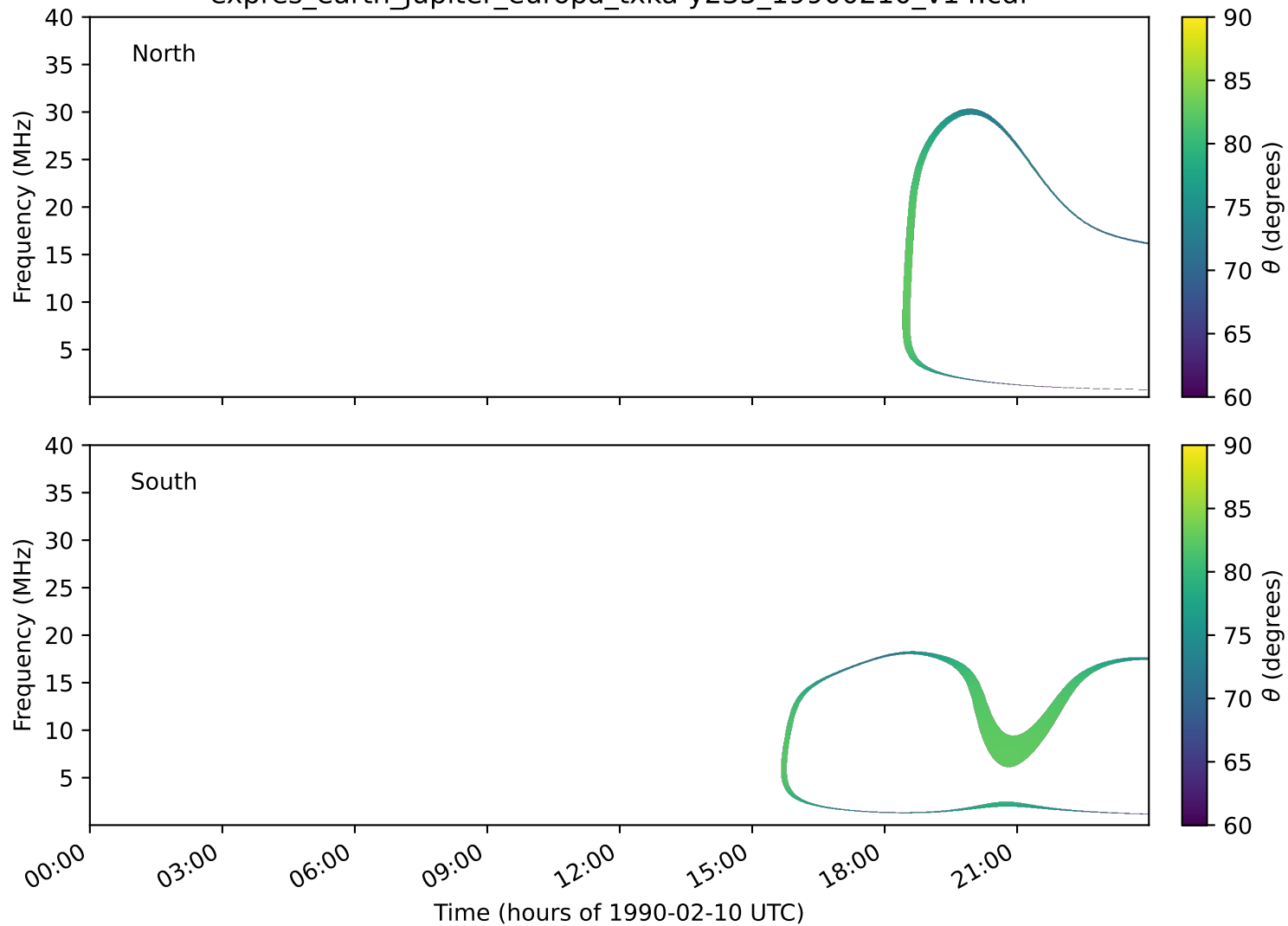
expres_earth_jupiter_europa_txka-y235_19900210_v14.cdf
