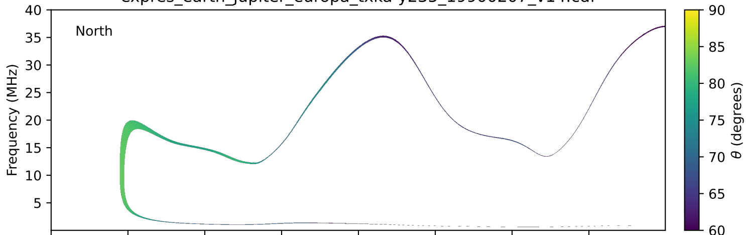
expres_earth_jupiter_europa_txka-y235_19900207_v14.cdf
