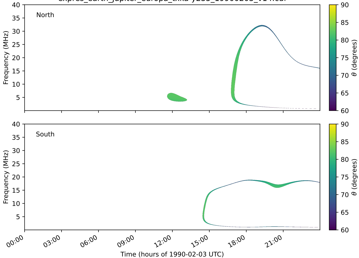
expres_earth_jupiter_europa_txka-y235_19900203_v14.cdf
