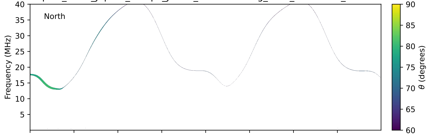
expres_earth_jupiter_europa_jrm33_lossc-wid1deg_3kev_19900218_v11.cdf
