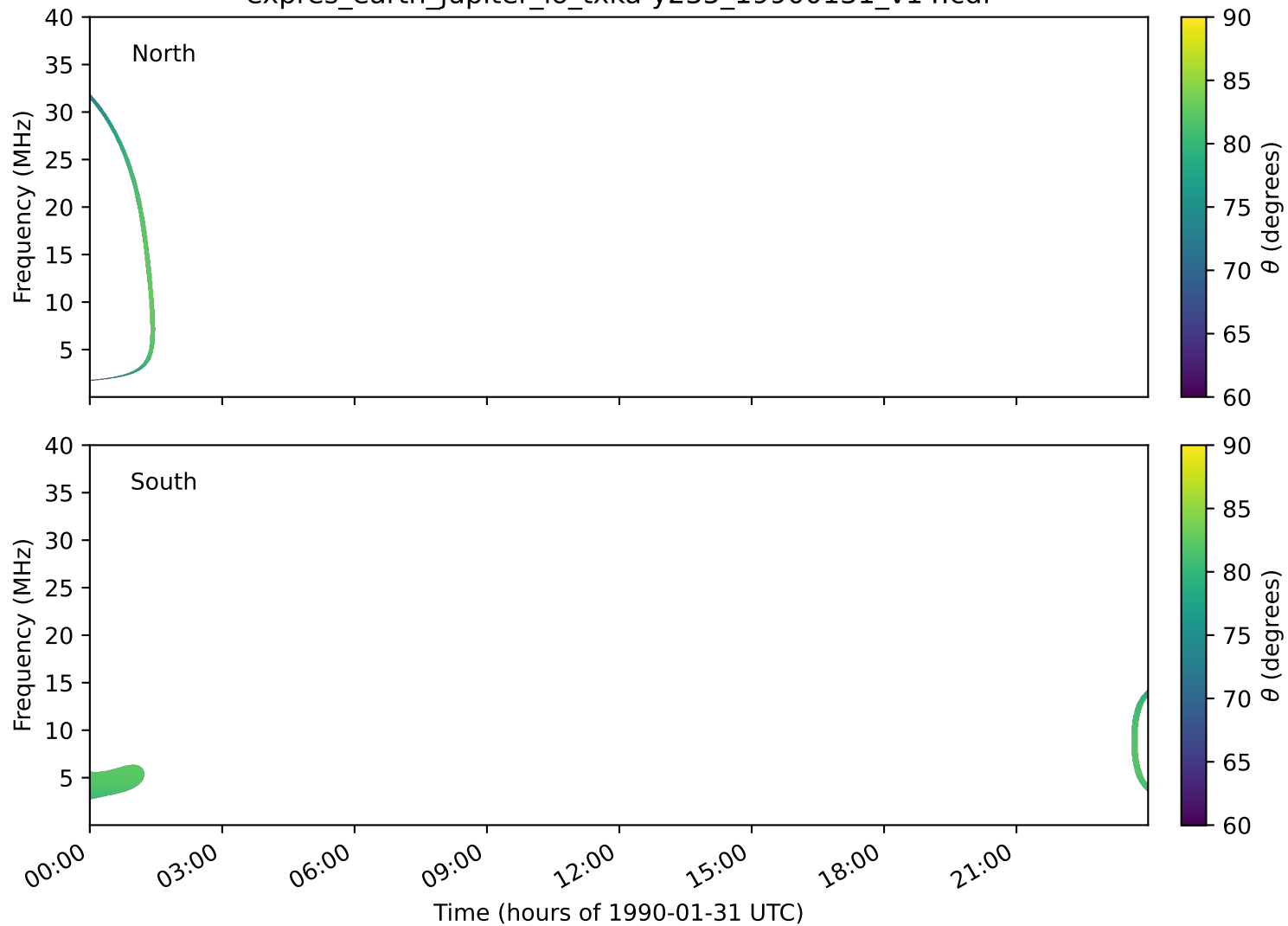
expres_earth_jupiter_io_txka-y235_19900131_v14.cdf
