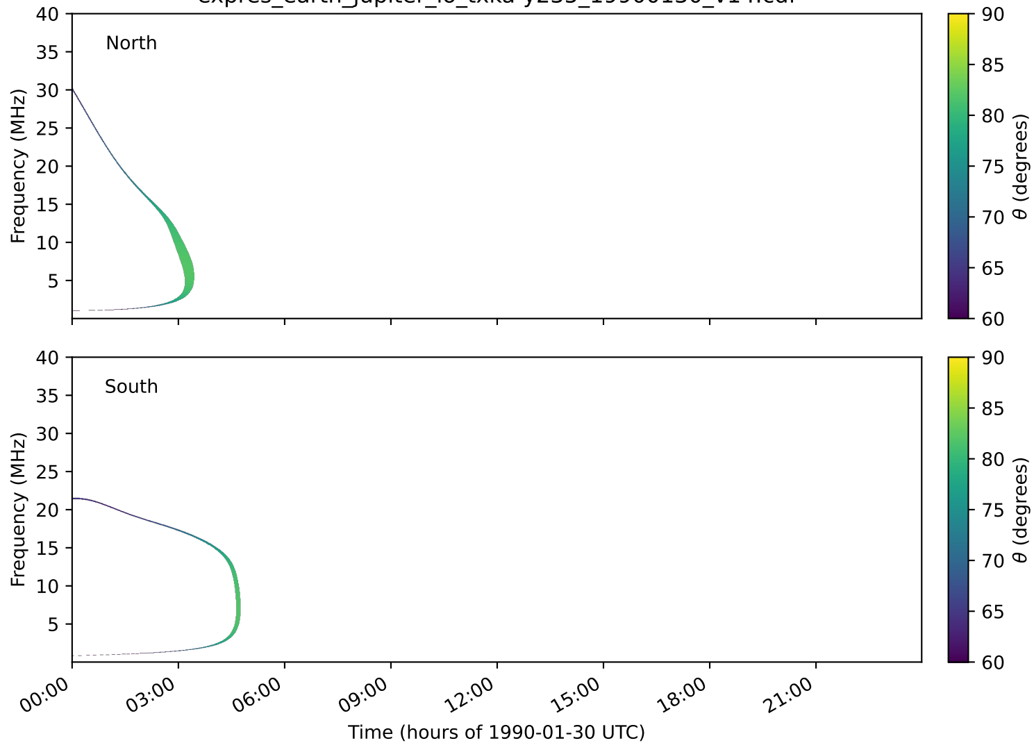
expres_earth_jupiter_io_txka-y235_19900130_v14.cdf
